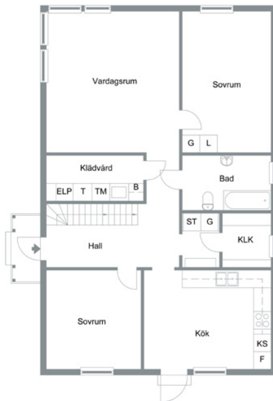
Bottenplan
